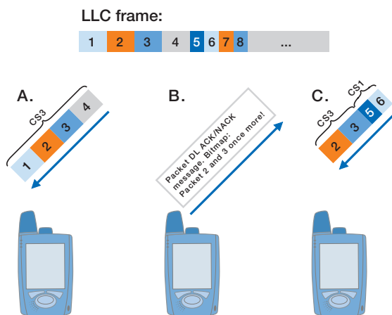
Figure 5. Packet transfer and retransmission for GPRS. (Legend: ACK/NACK, acknowledged/unacknowledged; CS, Coding Scheme)
