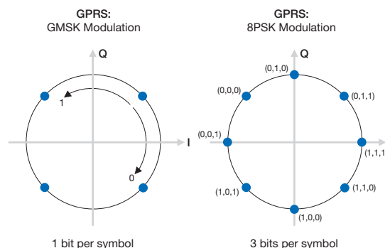
Figure 3. I/Q diagram showing EDGE modulation benefits.
